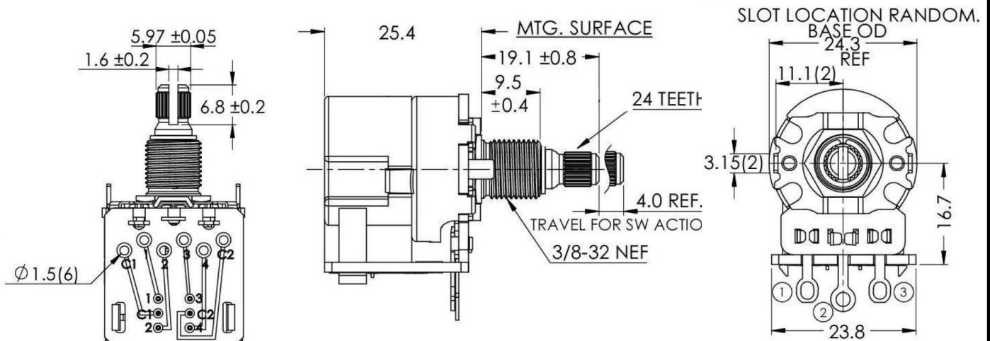
SWITCH DIAGRAM
