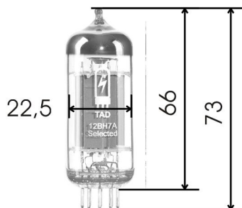
Outline View
